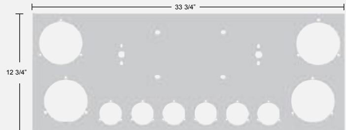
Rear panel are enclosed on all sides, steel backing plate included
